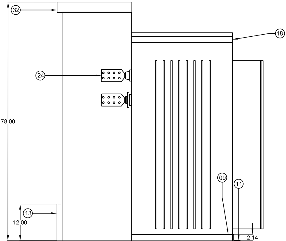
SIDE VIEW WITH CABINET DOORS AND SIDES REMOVED
