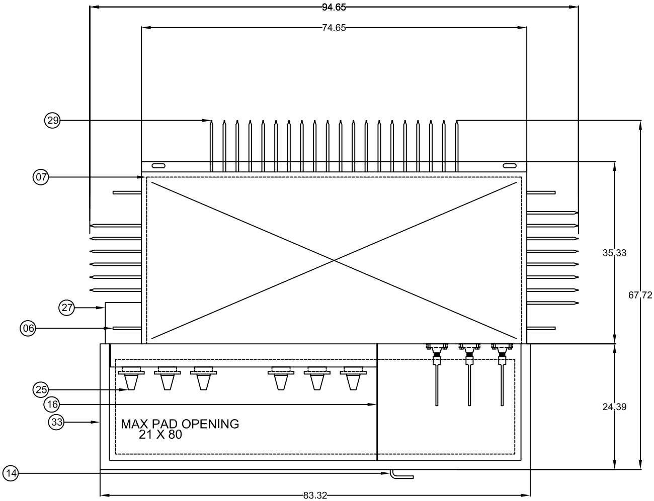
TOP VIEW WITH CABINET COVER REMOVED
