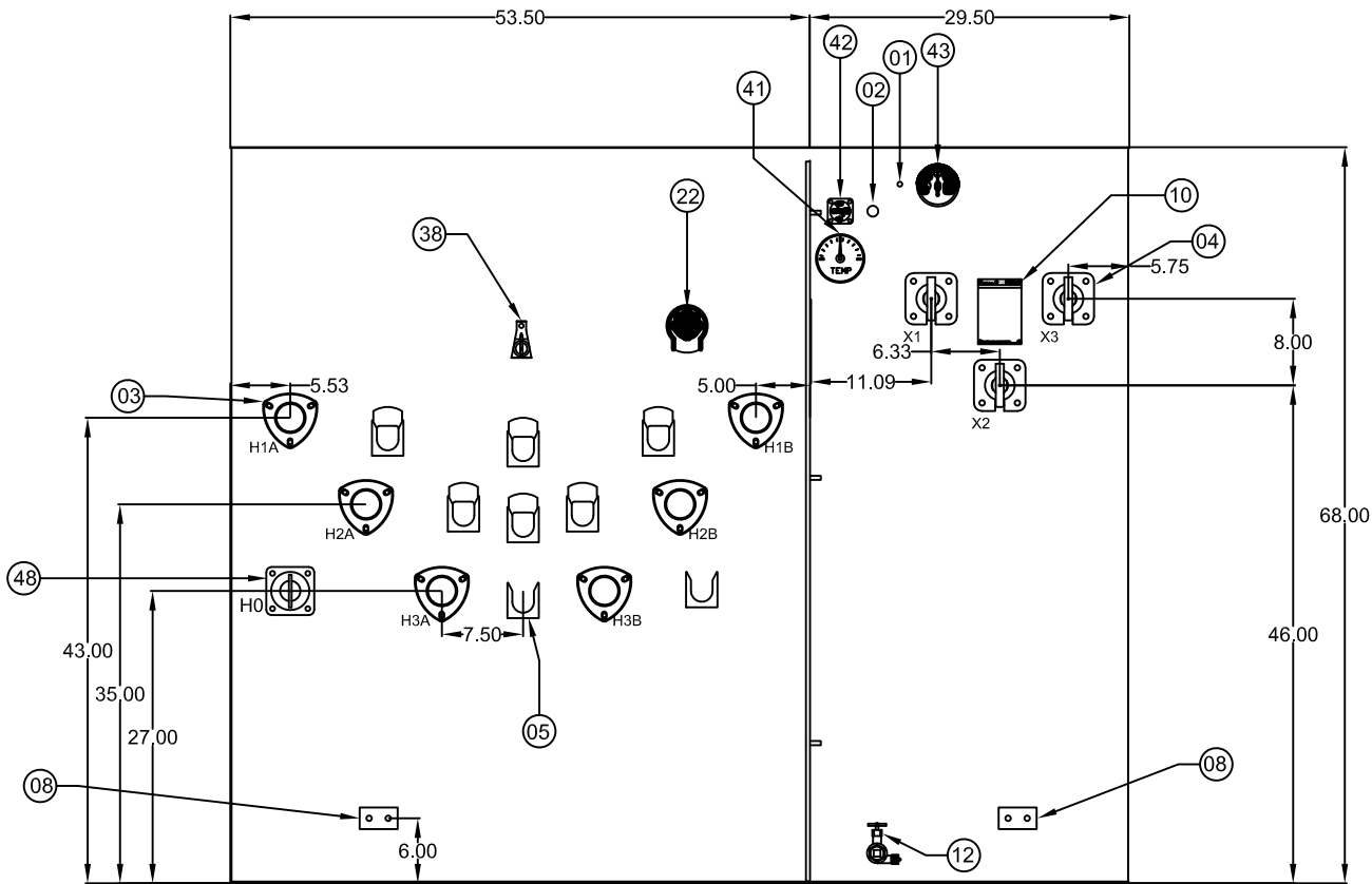
FRONT VIEW WITH CABINET REMOVED
